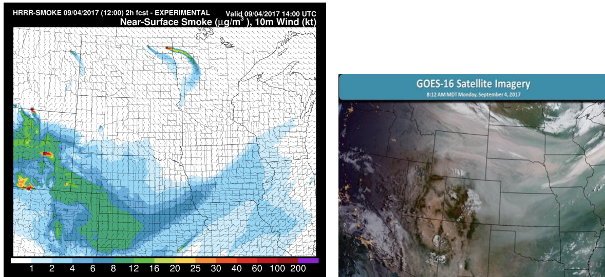
Fig. 49. Near-surface smoke. (left) From HRRRX (with 10-m wind) for a case of widespread western U.S. fires on 4 September 2017. GOES-16 GeoColor imagery (right) shows the observed extent of smoke in the atmosphere, which is likely more comparable to the HRRR forecast product shown below.
