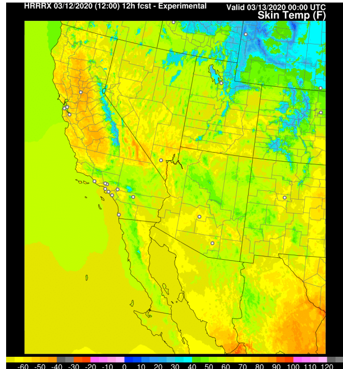
Fig. 14. Skin temperature. From 12-h forecast valid 00z/13 Mar 2020 from the 12z/12 Mar HRRRX. Graphic in °F.
