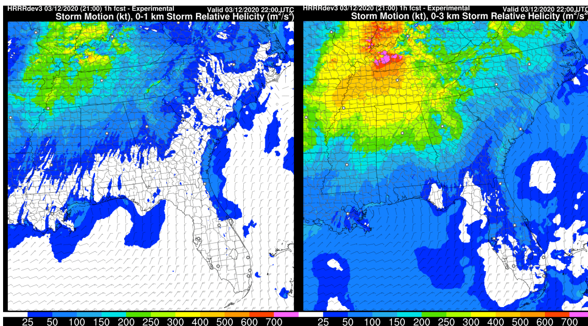
Fig. 31. Storm-relative helicity (SRH, in m^2 s^{-2} ) fields displayed with calculated storm motion. 0-1 km AGL SRH (left) and surface-to-3km AGL SRH (right). Shown are 1-h forecasts from HRRRX valid at 22z/12 March.
